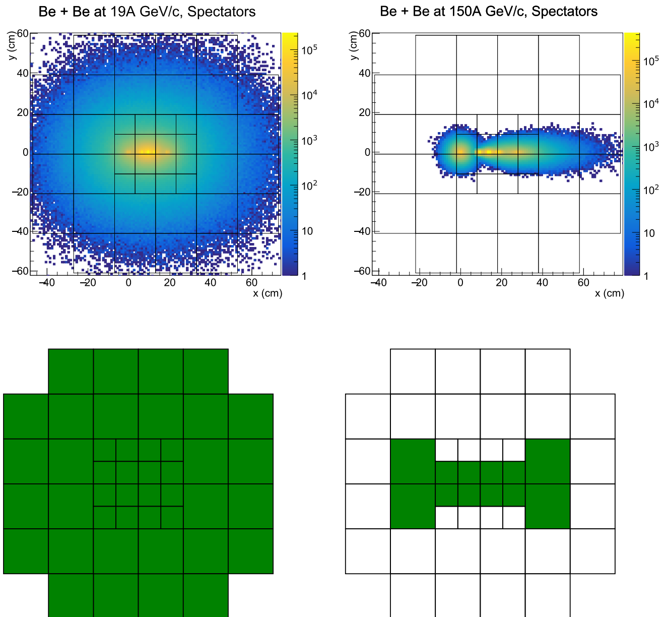
Fig. 6 Upper row: Simulated impact points of particles on the front face of the PSD for beam momentum of 19A GeV/c (left) and 150A GeV/c (right). Lower row: PSD modules included in the calcu-
